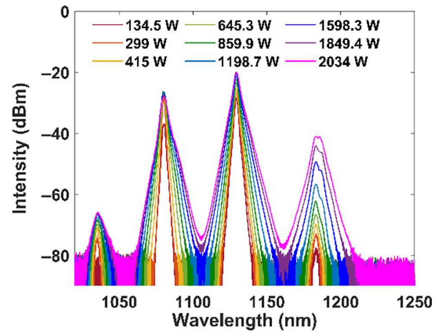
Figure 3. The spectrum of a Raman amplifier for various signal laser power outputs.
